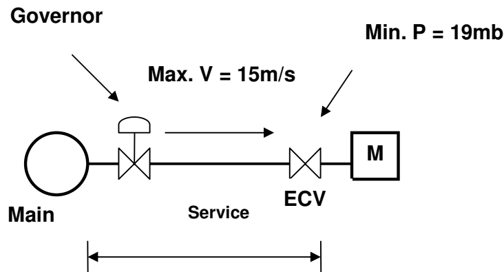
Figure B.2: Service with Remote Pressure Reduction
